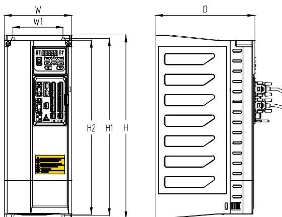
б) GK900-4T18.5LB – GK900-4T45L(B)
